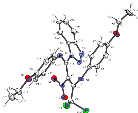
Fig. 3. Molecular structure of ( E,E )-1-(benzotriazol-1-yl)-4,4-dichloro-3-(4-ethoxyphenyl-amino)-1-(4-ethoxyphenyl-imino)-2-nitrobut-2-ene ( 30 ) in the solid state.
